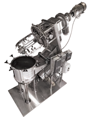
High-Shear Mixers
